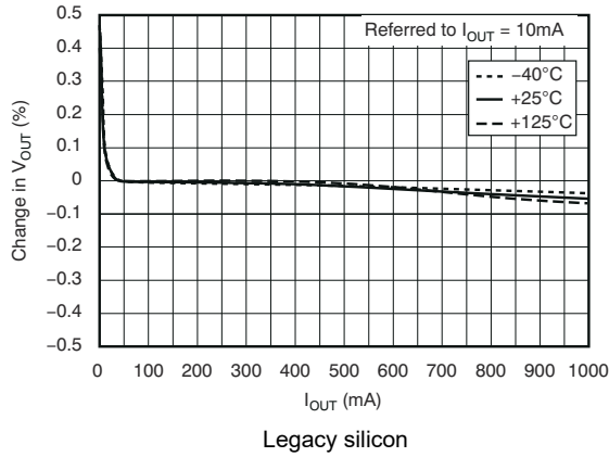
Figure 5-1. Load Regulation
