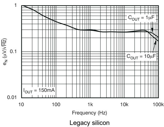
Figure 5-27. Noise Spectral Density
