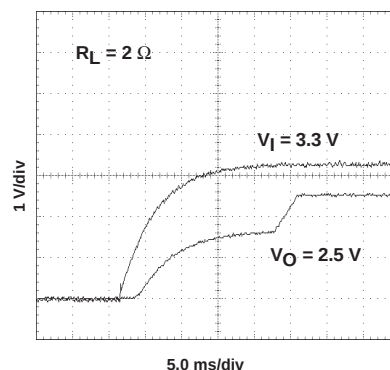
START UP WAVEFORM
