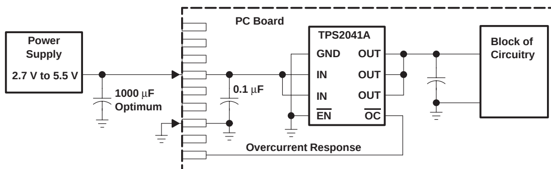
Figure 33. Typical Hot-Plug Implementation (Example, TPS2041A)
