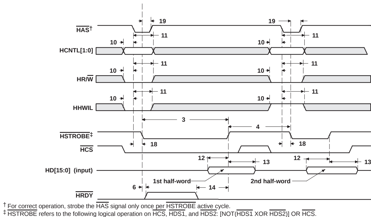
Figure 7-33. HPI16 Write Timing ( \overline{\text{HAS}} Used)
