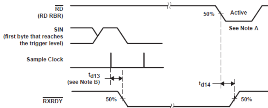
Figure 6-7. Receiver Ready ( \overline{\text{RXRDY}} ) Waveforms, \text{FCR0} = 0 or \text{FCR0} = 1 and \text{FCR3} = 0 (Mode 0)
