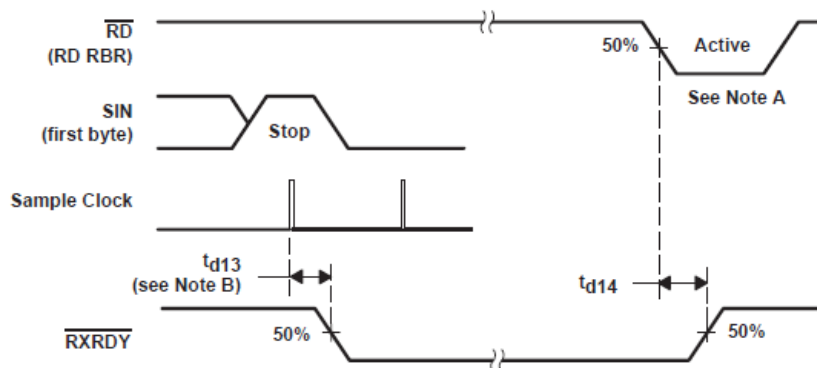
Figure 6-7. Receiver Ready ( \overline{\text{RXRDY}} ) Waveforms, \text{FCR0} = 0 or \text{FCR0} = 1 and \text{FCR3} = 0 (Mode 0)
