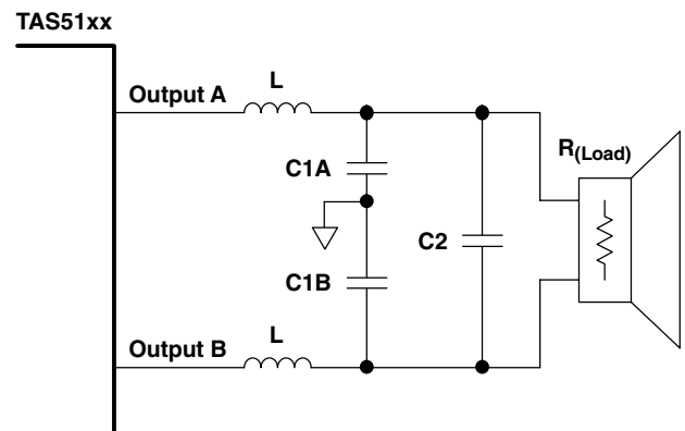
Figure 12. Demodulation Filter
