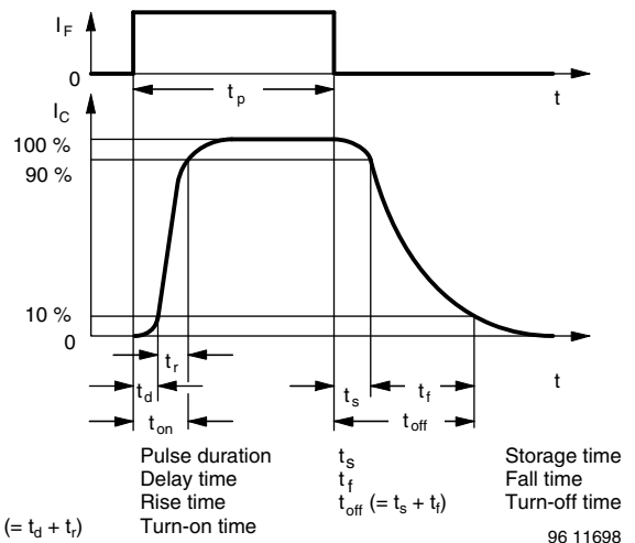
Fig. 3 - Switching Times
