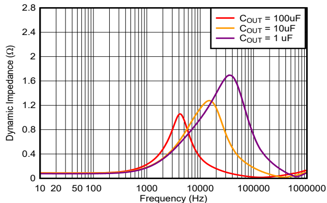
Figure 6-40. Output Impedance
