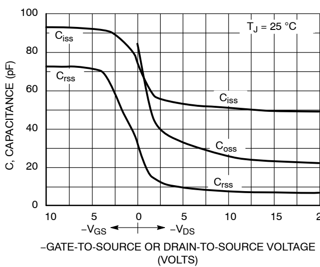
Figure 7. Capacitance Variation
