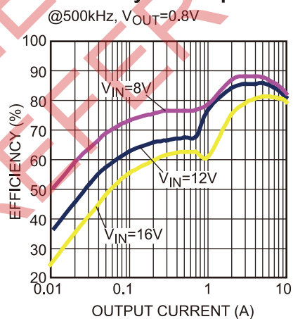
Figure 24 — Efficiency Curve
