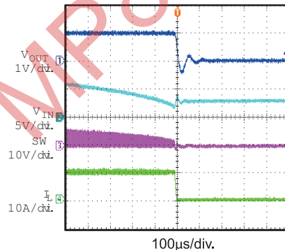
Shutdown Through I_{IN}
