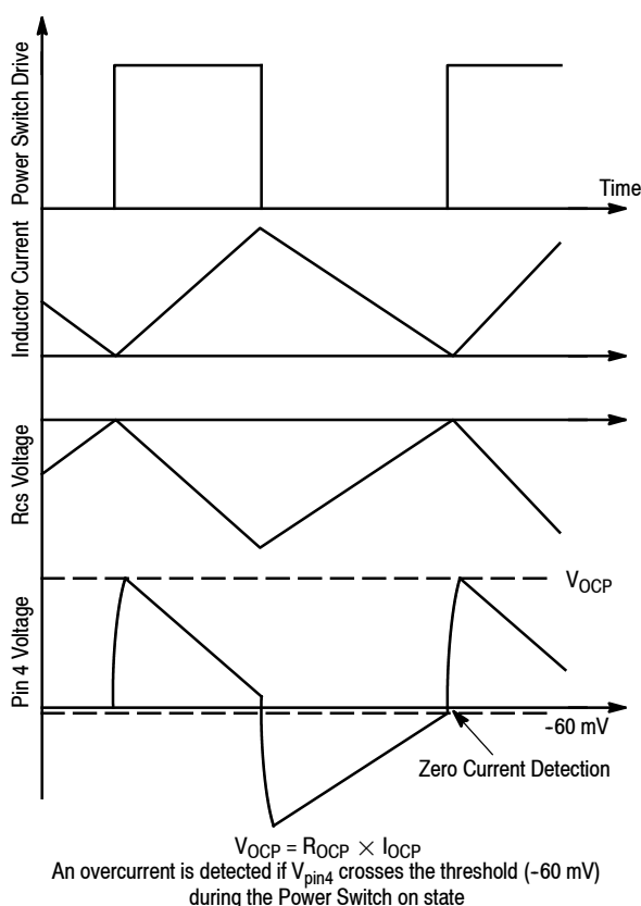
Figure 27. Current Sensing
