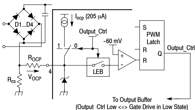
Figure 28. Current Sense Block
