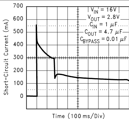
Figure 5-3. Short-Circuit Current (Legacy Chip)
