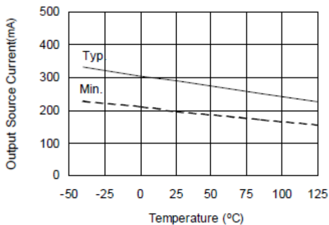
Figure 18A. Output Source Current vs. Temperature
