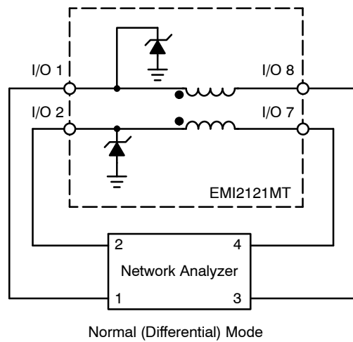
Figure 1. Normal (Differential) Mode Test Configuration
