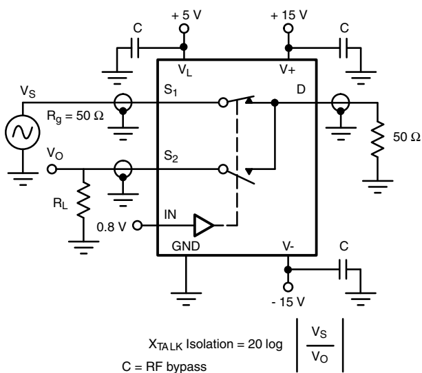
Fig. 6 - Crosstalk (DG419)
