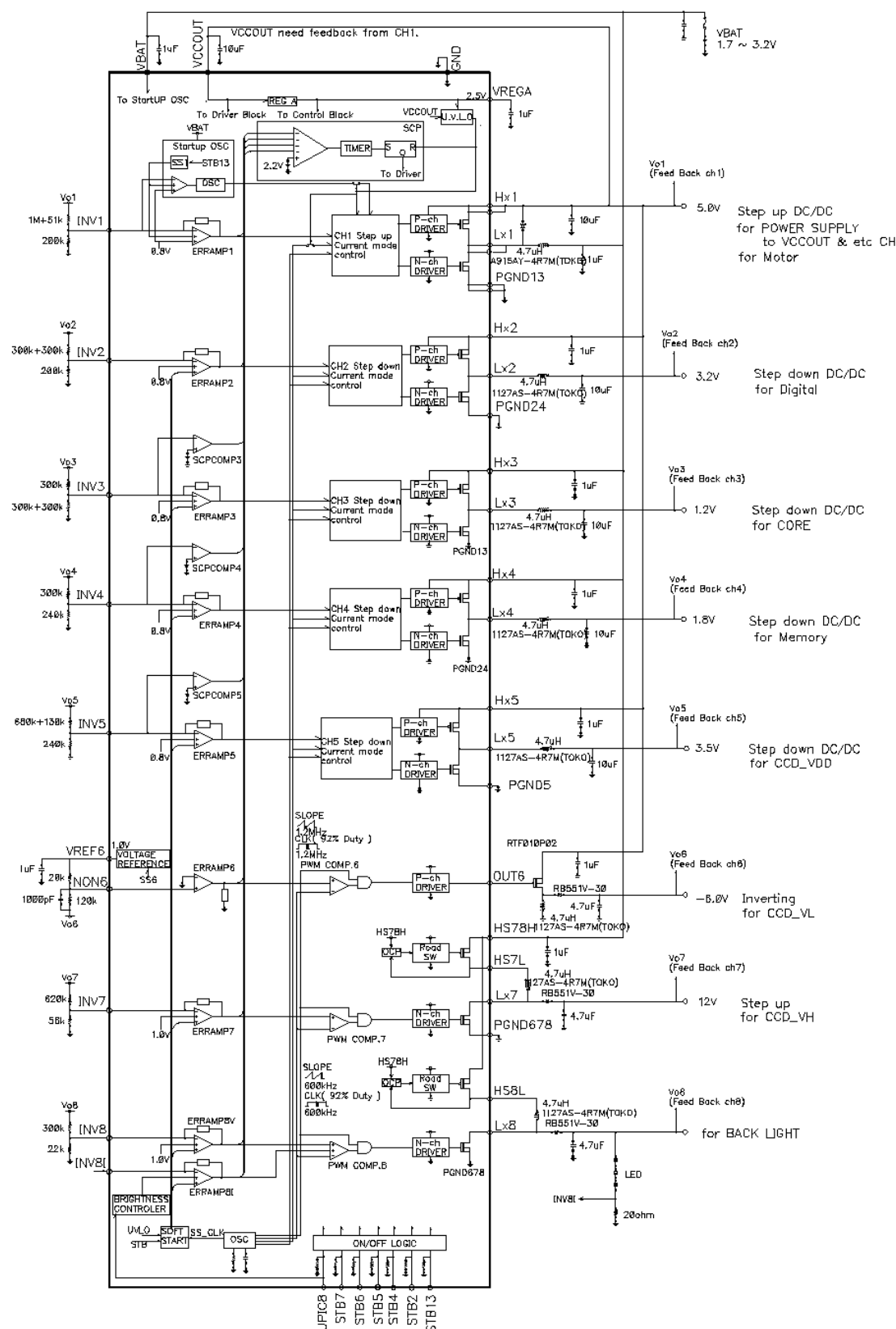
Fig.24 Applied circuit diagram 2(dry battery ×2)
