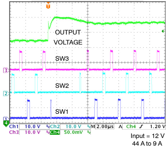
Figure 12. Load Transient
