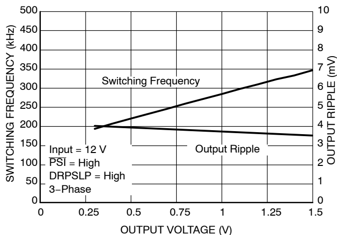
Figure 25. Switching Frequency in PWM
