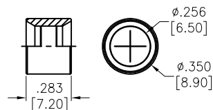
Ⓓ Seal
