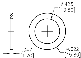
Ⓑ Washer
