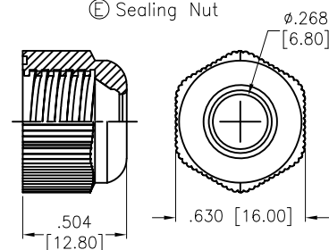
Ⓔ Sealing Nut
