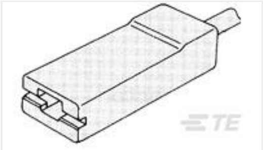
TE Part #1-480416-8 250 FASTON HSG.,REC.,1 POS, NATURAL
