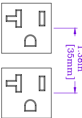
VIEW C
