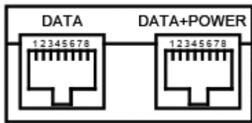
J1 Pins J2 Power: 4, 5(+) J2 Pins 7, 8(-)
