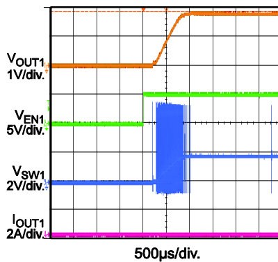
Enable On without Load
