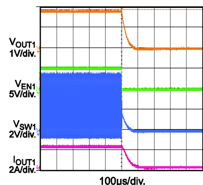
Enable Down with 2A Load
