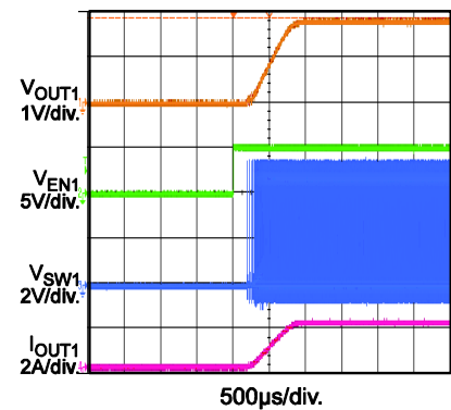
Enable On with 2A Load
