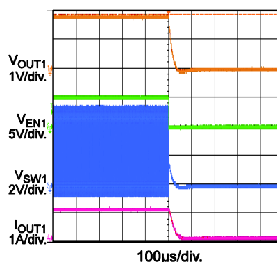
Enable Down with 1A Load
