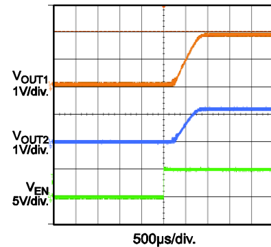
EN On with 2A Load
