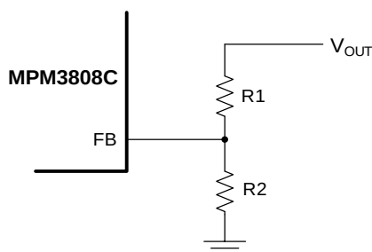
Figure 4: Feedback Network
