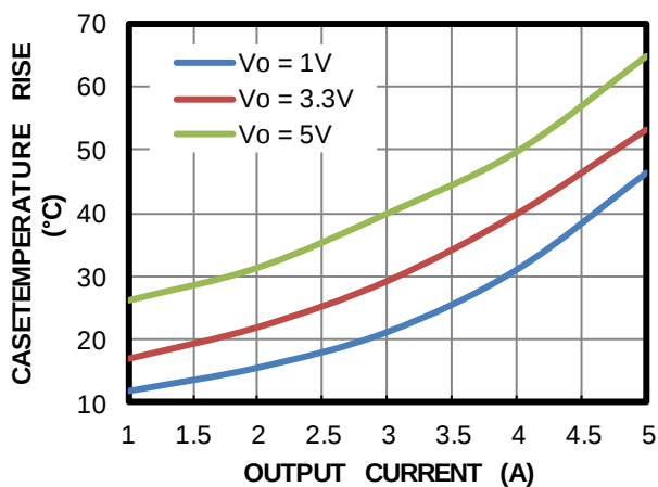
Output Current vs. T_{RISE}
