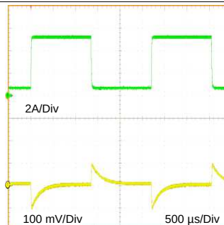
Figure 44. Transient response
