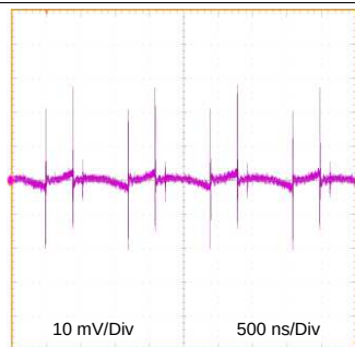
Figure 43. Output ripple
