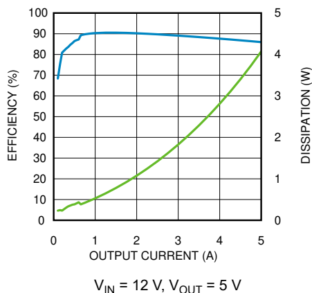
Figure 7-4. Efficiency
