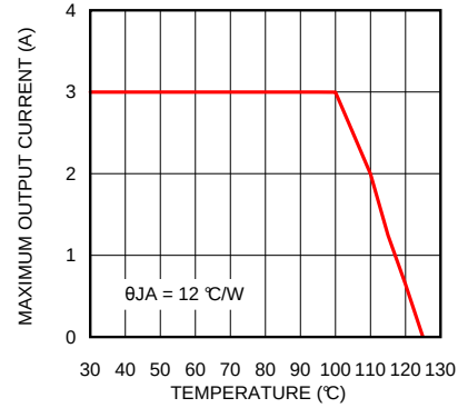
Figure 38. Thermal Derating
