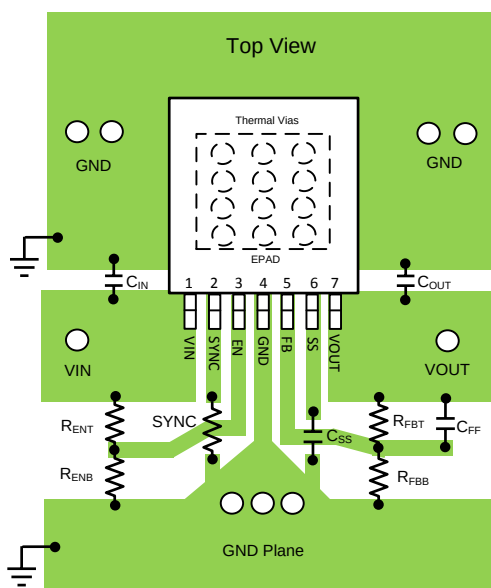
Figure 53. PCB Layout Guide
