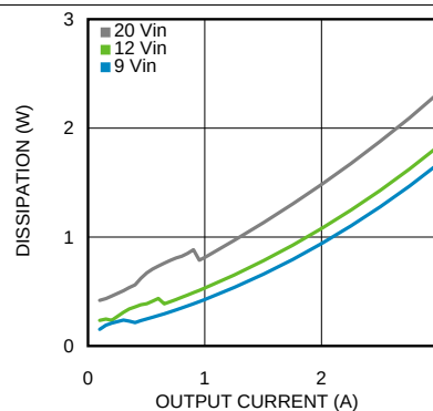
Figure 2. Dissipation 6-V Output at 25°C Ambient
