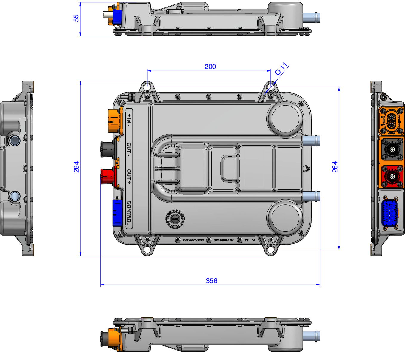
Figure 7. Mechanical Drawing
