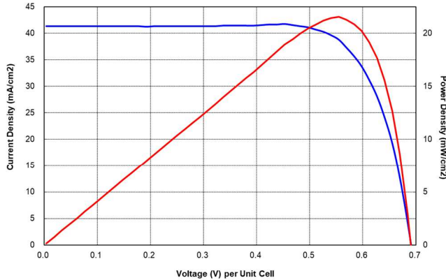
Current-Voltage Characteristics
