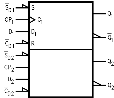
Figure 3. Logic Symbols
