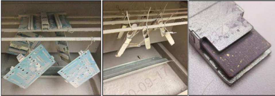
Figure 1- Specimens Following Dust Exposure
