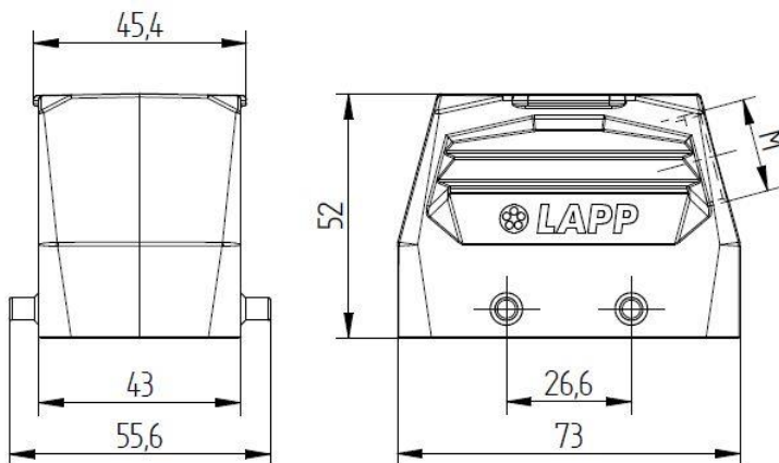
Side cable entry
