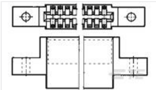
TE Part #583718-9 TW-LEAF CRP HSG 22 POS 100 C/L
