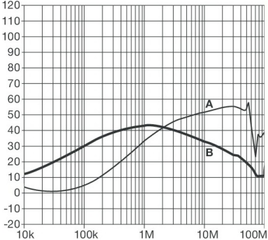
6 A B-types
