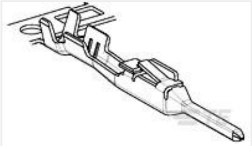
TE Part #171699-1 070 TYPE LOOSE PIECE REC CONT
