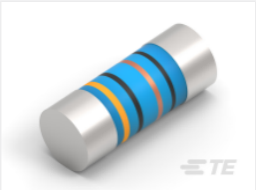
TE Part #7-2176315-0 MELF SMA_A 47K 1% 50PPM 0204 0.4 W
