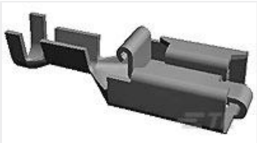
TE Part #880645-1 PL REC 1.0-2.5 MM2 0.40 X 52.32 BR
