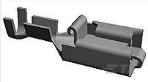
TE Part #880645-6 PL REC 1.0-2.5MM2 0.40 X 52.32 PTPBR
