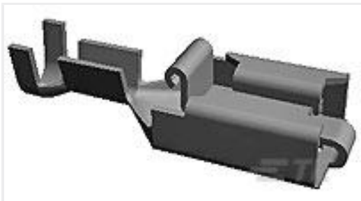
TE Part #880646-5 PL REC 0.5-1.0 MM2 0.40 X 52.32 PTPBR
