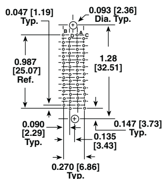
44 CONTACTS
