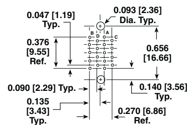
18 CONTACTS
