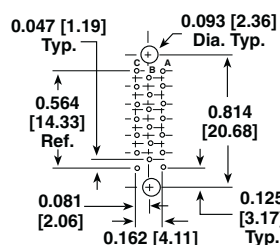
20 CONTACTS
