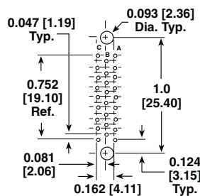
26 CONTACTS
