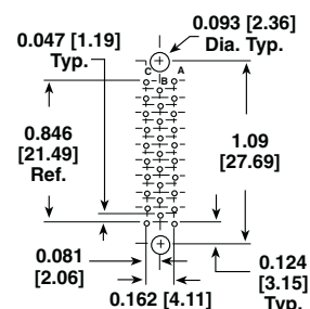
29 CONTACTS
