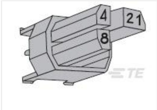
TE Part #5-100525-4 CODING DEV INSRT COLOR GREEN
