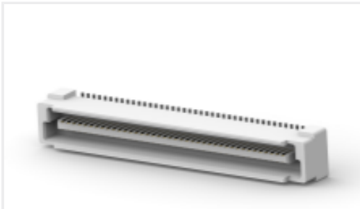
TE Part # 2-5179230-3 0.8FH,P06H.5,080,08/Sn,TU,SC
