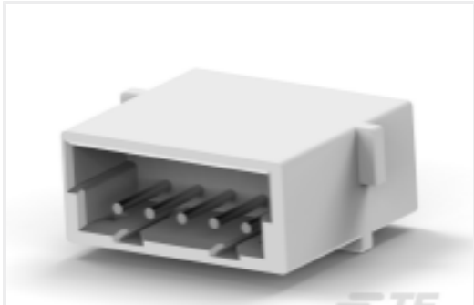
TE Part #CAT-3980655-RHAFH CT Relay Header Assembly: Free Hanging
