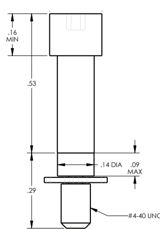
#4/40 M83513/05-15
