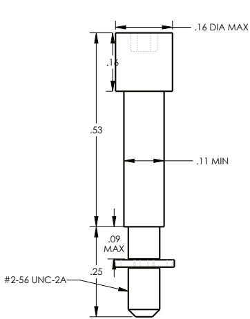
#2/56 M83513/05-05
