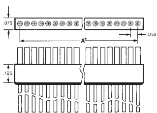
Socket Connector
