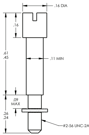
#2/56 M83513/05-06
