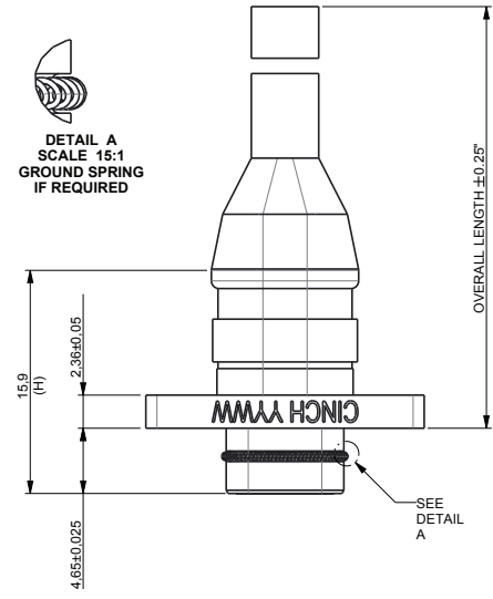
Plug Connector
