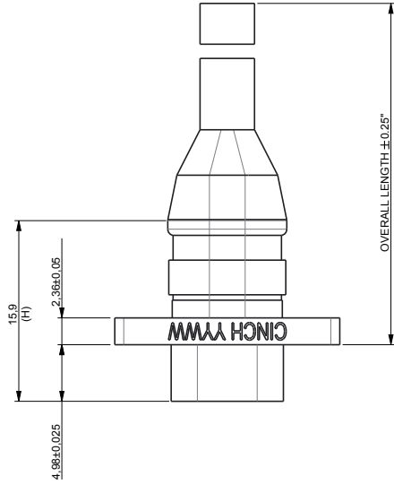
Socket Connector
