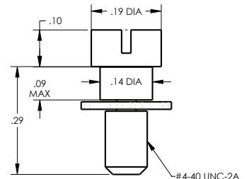
#4/40 M83513/05-13
