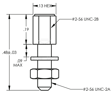
#2/56, Front Mount DCJP9-51
