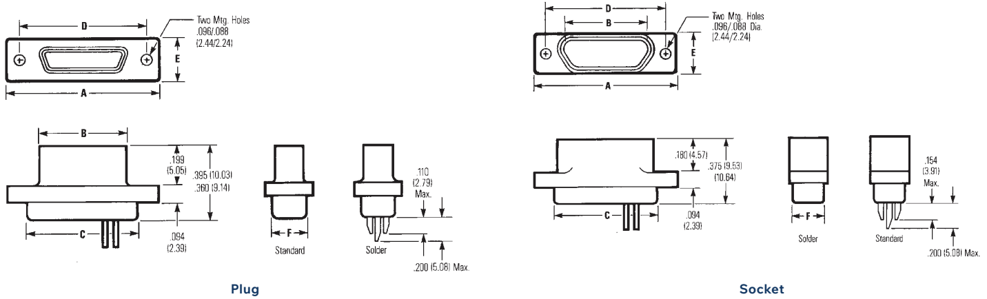
Plug
