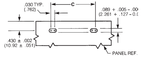
Figure 3: Edgeboard Mounting
