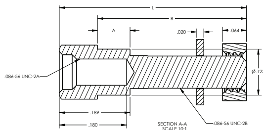
#2/56 Thread, Rear Mount DCJPRM0xx (See Table Below)
