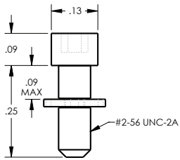
#2/56 M83513/05-02
