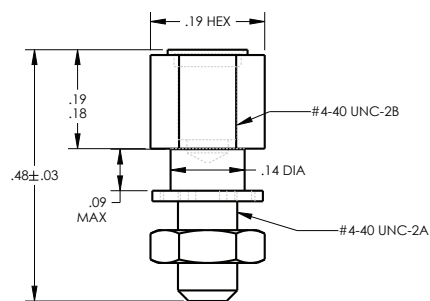
#4/40, Front Mount DCJP100
