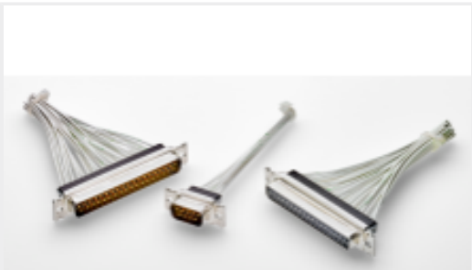
TE Part #2335890-2 AMPLIMITE SZ 2 RECEP 15 POS, ST STL SHEL
