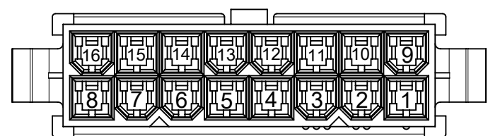
16 CKTS.
