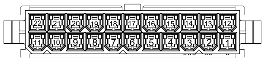
22 CKTS.
