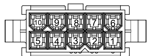
10 CKTS.
