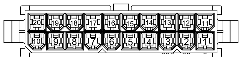
20 CKTS.
