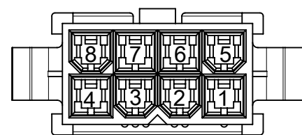
8 CKTS.
