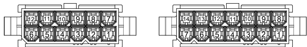
12 CKTS.
