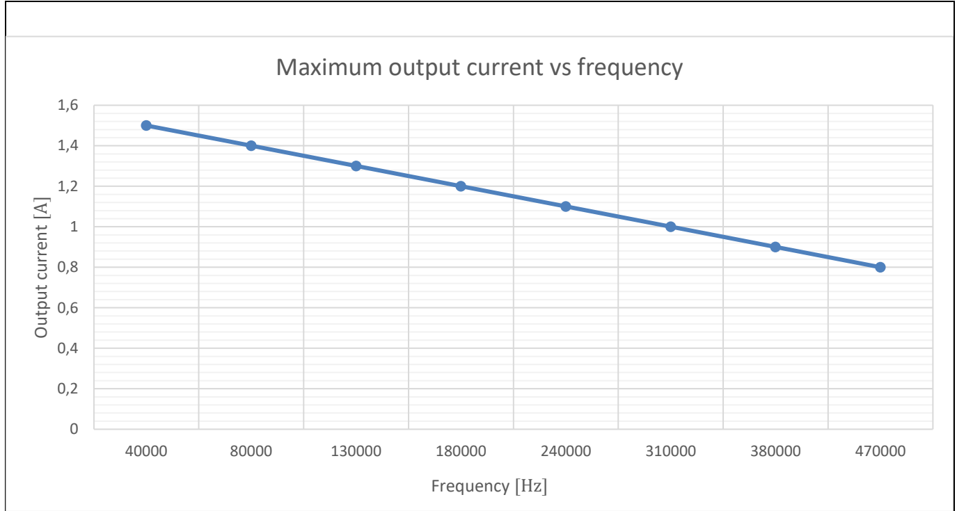
Figure 2 IC maximum output current capability at different frequencies with limited dissipated power, 0.98 W, and cooling area of 600 mm 2
