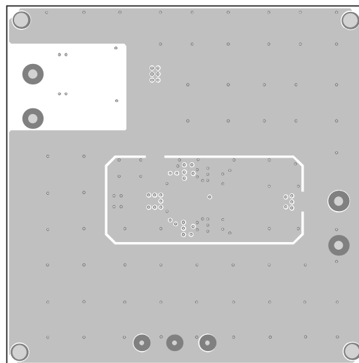
Figure 4: Mid-Layer 1
