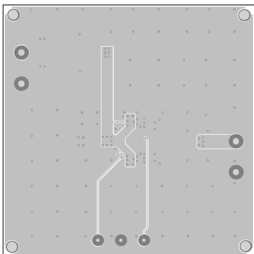
Figure 5: Mid-Layer 2
