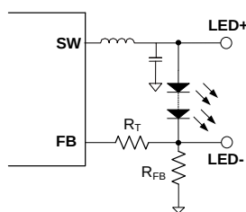
Figure 1: Feedback Network
