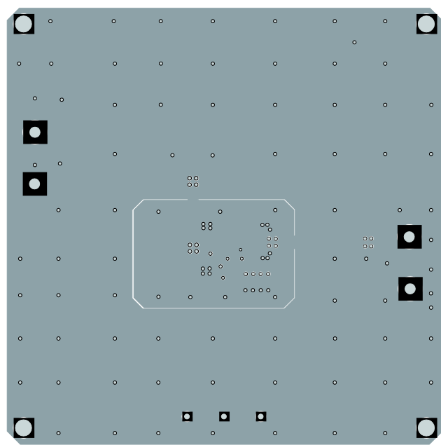
Figure 3: Inner1 Layer
