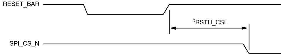
Figure 57. Reset to SPI Access Delay
