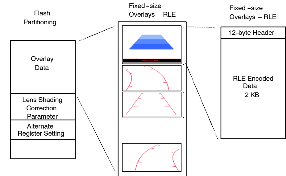
Figure 36. Memory Partitioning
