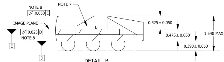
DETAIL B
