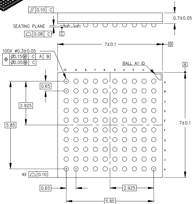
VFBGA100 7x7 CASE 138AH ISSUE O
