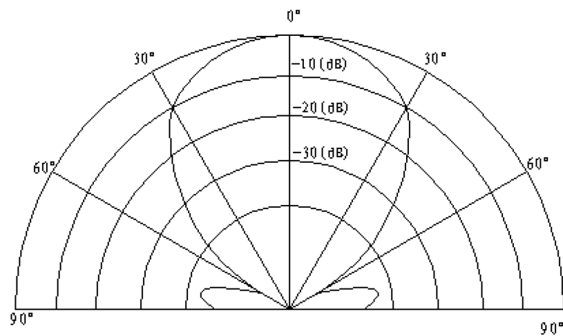
Directivity
